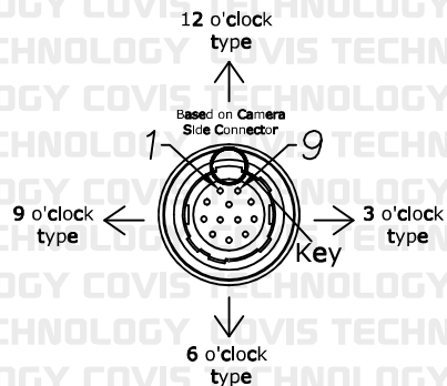
Camera Connector 3 o'clock type
